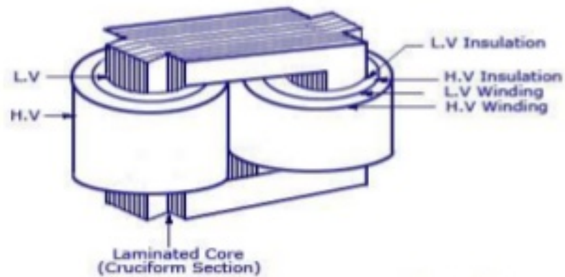
Core Type Transformer Cruciform Section
