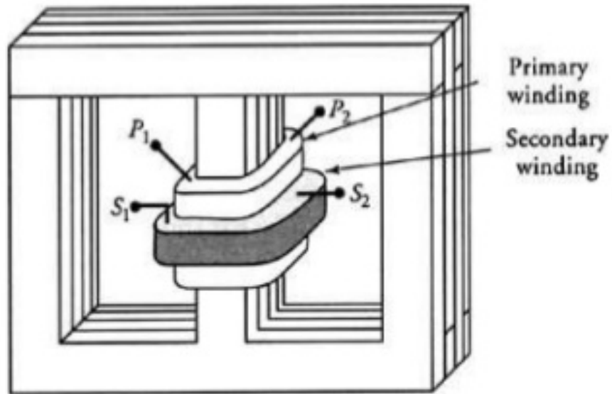
Core Type Transformer Cruciform Section
